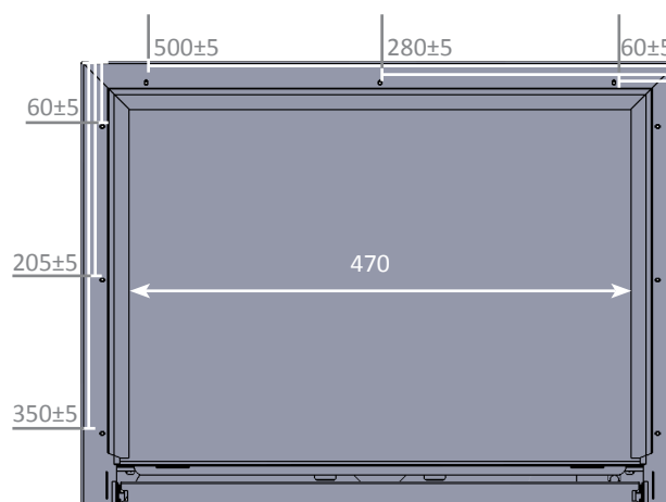
Dreamoc HD3 bottom - screw positions
