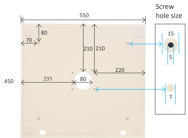
Dreamoc POP3B - bottom view measurements
